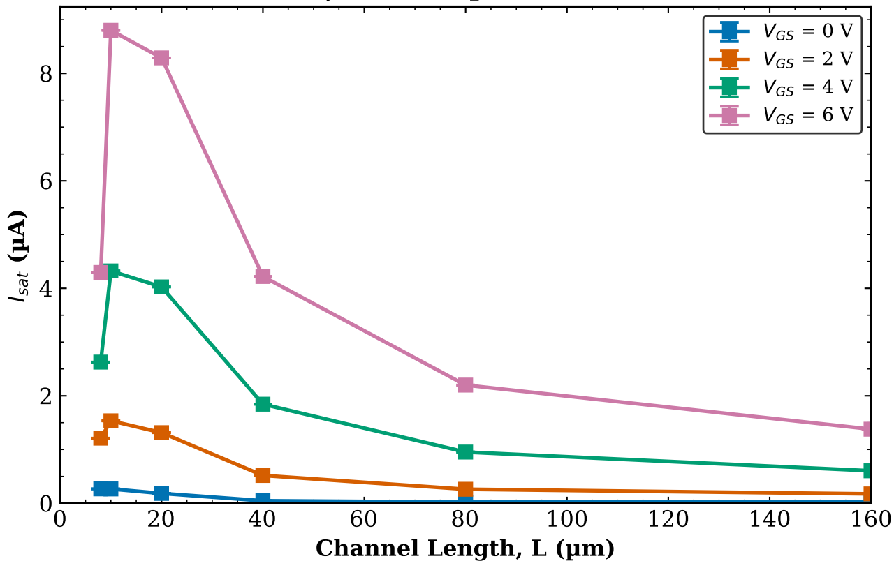
TFT1 Transistor 2 I_{sat} vs L | W = 10 \mu m (mean \pm std)
